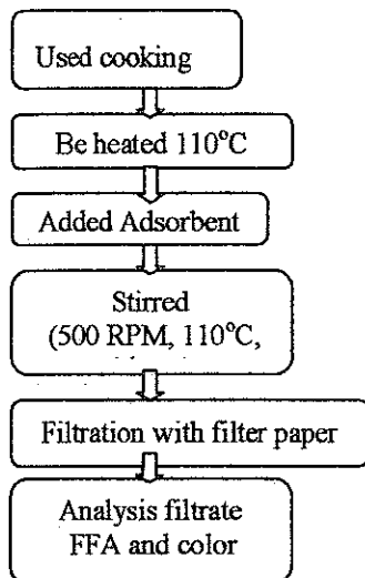
Figure 2: Flow Chart of Used Oil Purification Process
