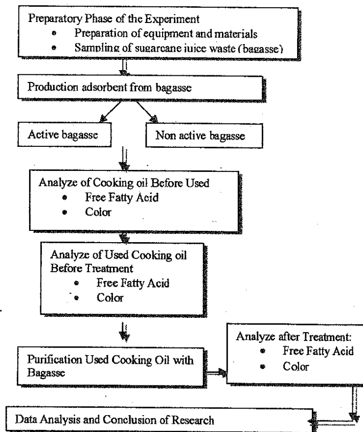
Figure 1: Flow Chart of Experiment
