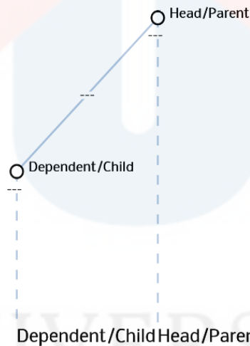
Figure 6: head-dependent attachment
